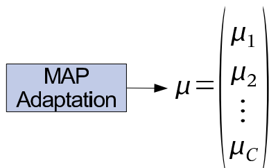
Figure 7.3: Illustration of the GMM supervector construction. All means of a single GMM are concatenated into a so called GMM supervector.
