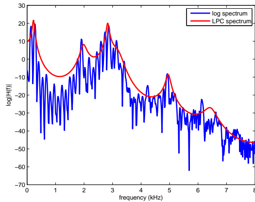
Figure 3.3: Example of a short voiced speech sample in the frequency domain. Representation of original log spectrum and corresponding formant frequencies by linear predictive coding.
