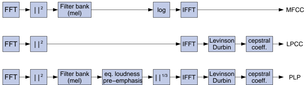
Figure 3.4: Comparison of different feature extraction methods used in this thesis: MFCC, LPCC and PLP
